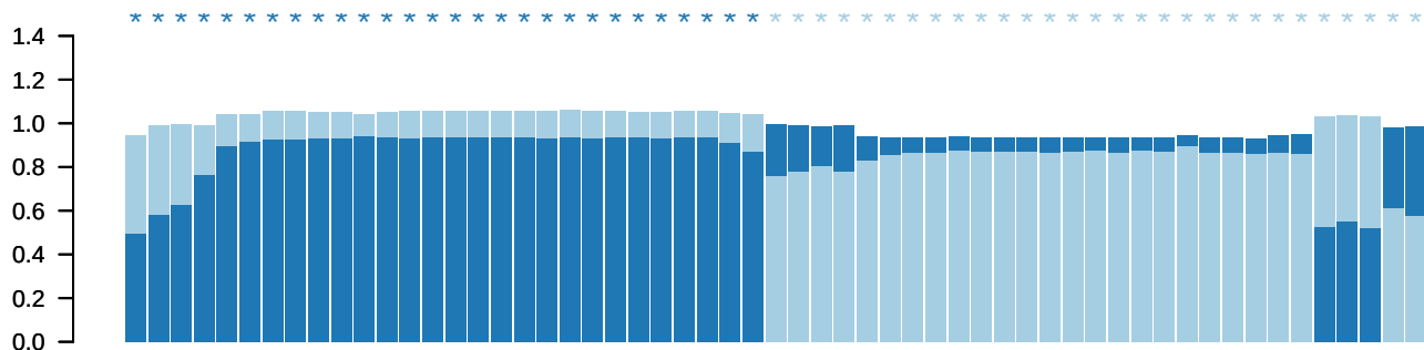
item-consensus
